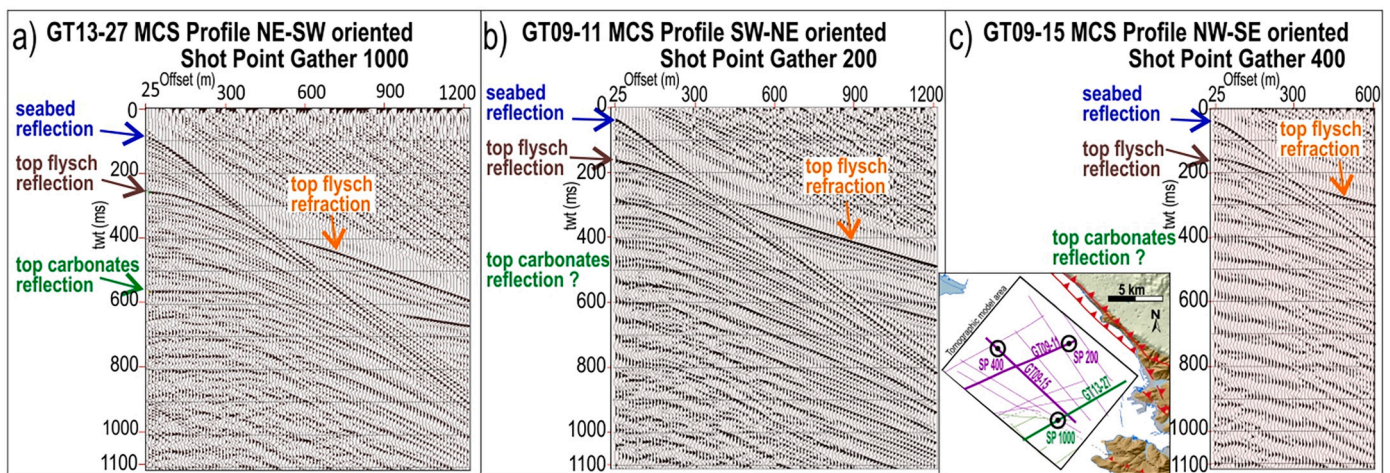
Fig. 3. Pre-stack raw data sorted by common shot gathers of MCS profiles a) GT13-27 (streamer length of 1200 m, 96 channels), b) GT09-11 (streamer length of 1200 m, 96 channels) and c) GT09-15 (streamer length of 600 m, 48 channels). Hyperbolas related to the reflection from the seabed and the top flysch and refraction from top flysch (blue, brown, orange arrows, respectively) can be identified with good certainty. Reflection from the top carbonates (green arrow) is hardly identifiable in 2009 pre-stack raw data, due to reverberations from shallow seabed and high reflection coefficient at top flysch surface. The inset map shows the location of the common shot gathers, displayed in a), b) and c), along their respective seismic profiles. (For interpretation of the references to colour in this figure legend, the reader is referred to the web version of this article.)
