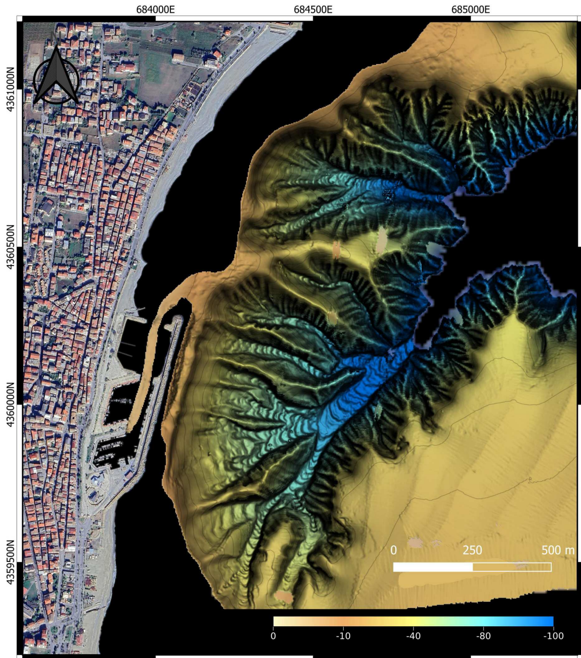
Figure 2. The headwall of the Cirò Marina canyon (1.5 km long and 50 m tall) incises the continental shelf up to a depth of 20 m, undermining the stability of the Cirò Marina harbour quay built in 2001. Storms, amplified by the steep morphologies of the canyon headwalls, are reported to recurrently damage the harbour infrastructure, which frequently requires repairs. To be noted the thalweg of the tributary channels of the Cirò canyon displays arcuate bedform morphologies, typically resulting from the activity of turbidity currents. These currents, which transport sediments downslope, can create distinctive bedforms on the seafloor, indicating cyclic episodes of sediment movement and deposition. The blended shaded relief map shows bathymetric data through a multilayered composition, including a color-coded depth map, multidirectional hill shading, and the application of the MSRM algorithm using the RVT software package (Novak et al., 2023).
